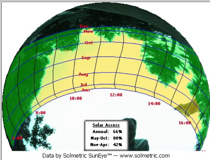
Monthly solar access: (Fixed; Tilt=18°; Azim=90°)
