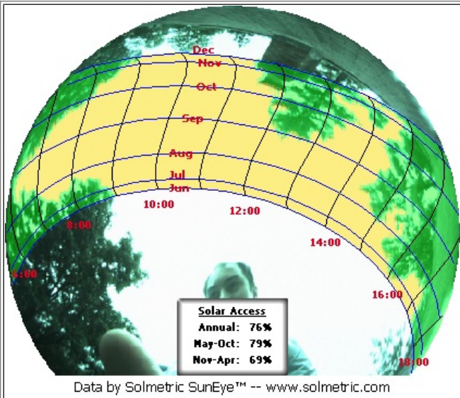
Monthly solar access: (Fixed; Tilt=18°; Azim=90°)
