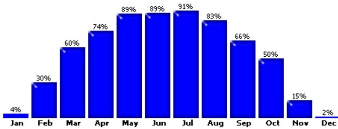
Monthly solar access: (Fixed; Tilt=18°; Azim=90°)
